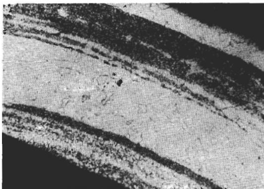
X 100. The heterogeneous nature of the steel from which the wire was drawn is apparent from the banding in the link
