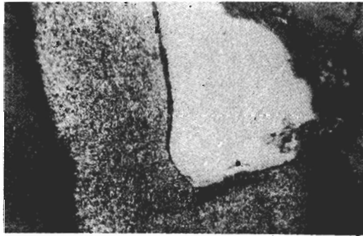
X 100 mag. Tempered martensite decarburised at joint
