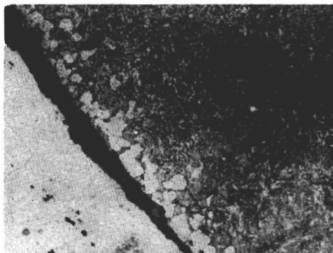
X 500. Martensite partly decarburised to ferrite at the joint
