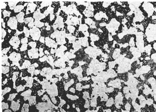
X 500. Ferrite and pearlite
