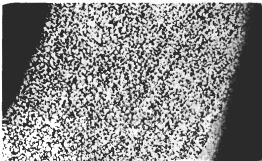
X 100. A fairly uniform mild steel
