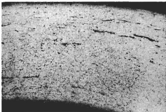
X 80. Ferrite and slag
