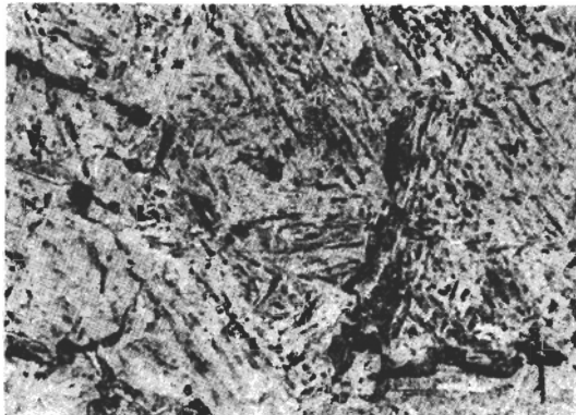
X 500. Martensite, with some bainite and ferrite
