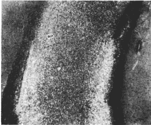
X 100 mag. Tempered martensite decarburised at joint
