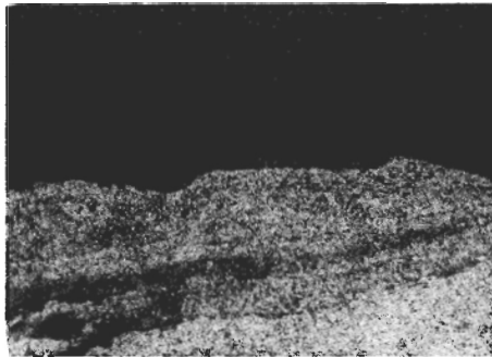
X 320. The decarburised area around the riveted joint. The low-carbon area is light-etching
