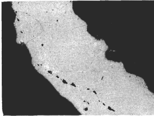
X 80. Ferrite and slag
